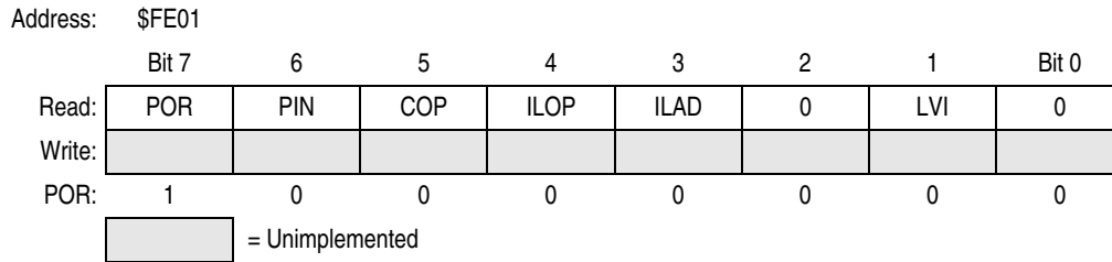
Figure 7-18. SIM Reset Status Register (SRSR)
