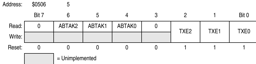
Figure 24-21. Transmitter Flag Register (CTFLG)
